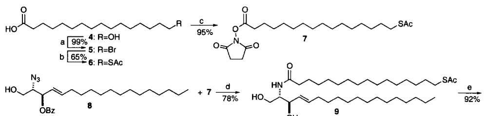
Scheme 1. a) HBr, AcOH, reflux, 3 d. b) AcSK, DMF, 60 °C, 8 h. c) N -hydroxysuccinimide, EDC, CH 2 Cl 2 , 12 h. d) MeONa, MeOH, 12 h, then pyridine, Et 3 N, MeOH, H 2 S, 22 °C, 16 h, then CH 2 Cl 2 , 7, Et 3 N, 22 °C, 12 h. e) MeONa, MeOH, 22 °C, 12 h.
