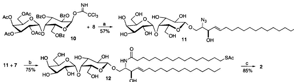
Scheme 2. a) CH 2 Cl 2 , MS 300 AW, BF 3 OEt 2 , 22 °C, 3 h, then MeONa, MeOH, 22 °C, 12 h. b) pyridine, Et 3 N, MeOH, H 2 S, 22 °C, 16 h, then CH 2 Cl 2 , 7, Et 3 N, 22 °C, 12 h. c) MeONa, MeOH, 22 °C, 3 h.
